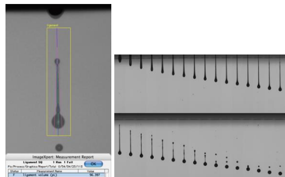
Figure 9: ImageXpert JetXpert drop-in-flight analysis tool [6]
