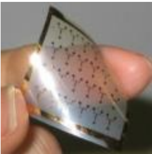
Figure 7: An ink jet-printed single-walled carbon nanotube (SWCNT) flexible thin-film transistor (TFT). [5]
