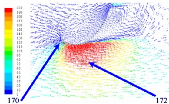
Figure 3: CFD of a C foil. From patent US 8188611.
