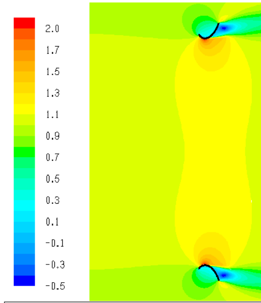
Figure 4: CFD of a C foil shroud with 10 meters diameter
