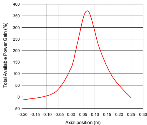
Figure 5: Percentage increase of power gain plotted against axial position of the propellers in relation to the shroud.
