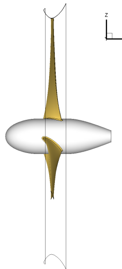
Figure 6: Blade and shroud combination
