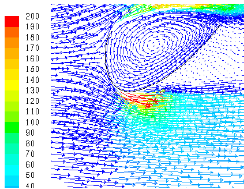
Figure 2: CFD of a funnel-like structure. Red is highest velocity; dark blue is the lowest.
