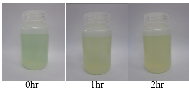
Figure 4: Color change of extraction solutions of alumina by the MgO modified soda sintering method
