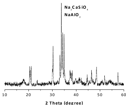
Figure 3: XRD spectra of sintered material at 1150°C for two hours by improved lime soda sintering method
