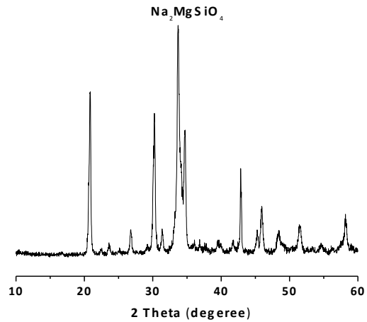
Figure 2. XRD spectra of sintered material at 1050°C for a half hour by MgO modified soda sintering method
