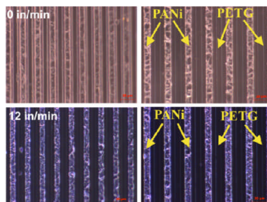
Figure 3: Optical micrographs showing the transfer of PANi on PETG surface at different belt speeds.
