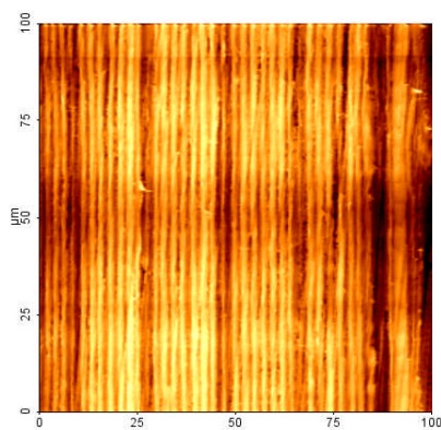
Figure 7: Horizontal nanolayered polymer film produced by multilayer co-extrusion.
