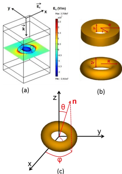
Figure 1. Photonic analysis, particle geometries and orientations: (a) computational domain and field analysis for a nanotorus, (b) nanoring (top) and nanotorus (bottom) geometries, (c) nanotorus and nanoring orientations [1, 2]
