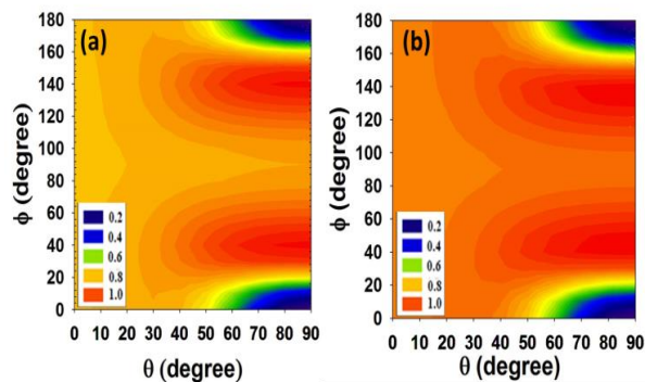
Figure 2. NIR absorption at a fixed LSPR wavelength as a function of orientation ( \theta and \phi ): (a) nanoring at \lambda=793\text{nm} ( r=20\text{nm} , R=40\text{nm} ), (b) nanotorus at \lambda=825\text{nm} ( r=10\text{nm} , R=30\text{nm} ).
