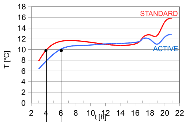
Figure 5: Average of the temperature recorded inside standard packaging and active packaging, respectively.
