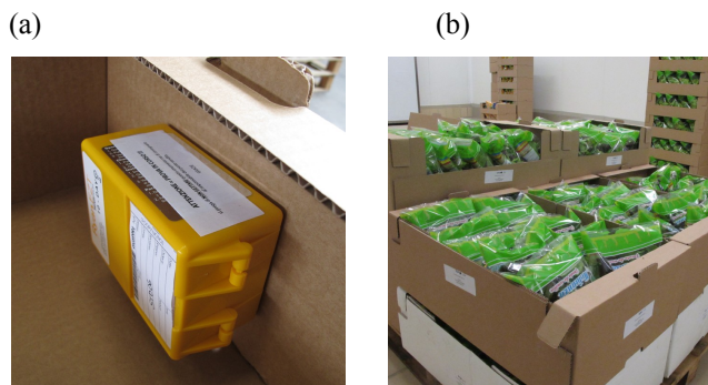
Figure 2: (a) Data temperature recorder (RYAN-SENSITECH, mod. EZT) placed inside each packaging; (b) Active and standard packaging monitored in the cold-store.
