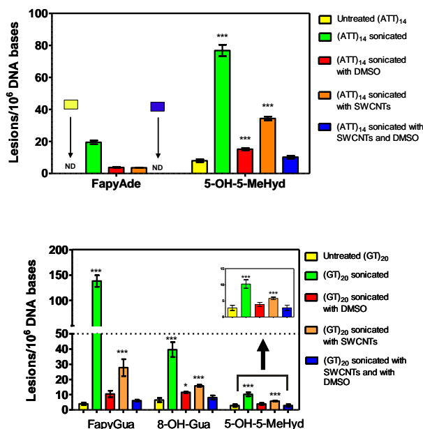
Figure 1. DNA damage evaluation by GC/MS of oligomers sonicated in the presence or absence of 0.1% DMSO and SWCNTs. Sonication time was 60 min. Two different oligomers were used: (ATT) 14 (upper) or (GT) 20 (lower). The ratio of DNA lesions/10 6 DNA bases represents the mean from five independent samples except for the DMSO only condition for (GT) 20 oligomer for which four samples were analyzed. The uncertainties represent standard deviations. Statistical analyses based on one-way ANOVA with posthoc Dunnett's multiple comparison test: * p value < 0.05; ** p value < 0.01; *** p value < 0.001. Reprinted with permission from [18].
