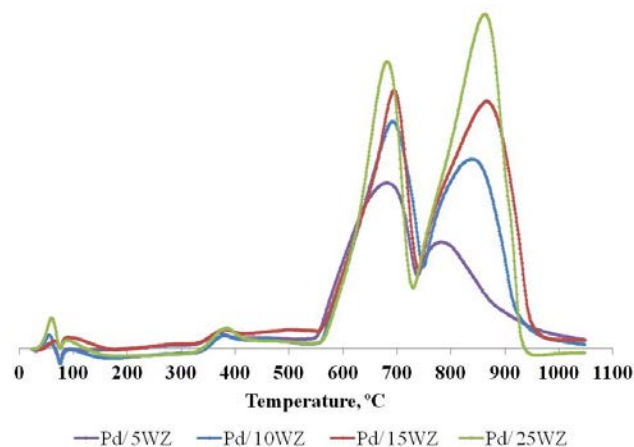
Figure 5. \text{H}_2 -TPR profiles of the PdO/ \text{ZrO}_2 - \text{WO}_3
