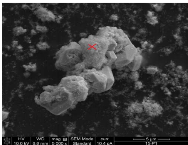
Figure 3. A STEM micrograph of the 1%Pd/15%WZ sample.
