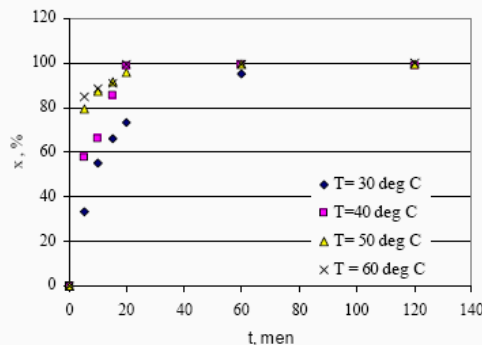
Fig 5. Effect of temperature on % conversion of oil (M = 4.5, C=4 %, N= 500 rpm)
