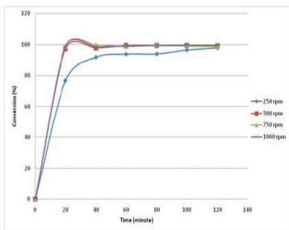
Fig. 4. Effect of stirring speed (rpm) on % conversion of oil (50 °C, M=4.5, C= 4 %)
