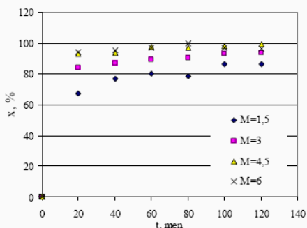
Fig.3. Effect of molar ratio of methanol to oil on % conversion (T=50 °C, C=4 %, N= 500 rpm)
