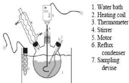
Fig. 1. Diagram of Methanolysis Equipment
