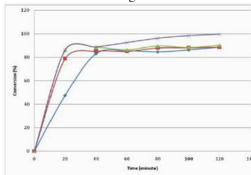
Fig.2. Effect of catalyst concentration on % conversion of oil (50 °C, N= 500 rpm)
