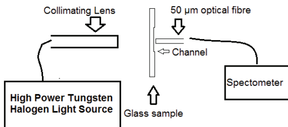
Figure 1: Transmission experimental set up
