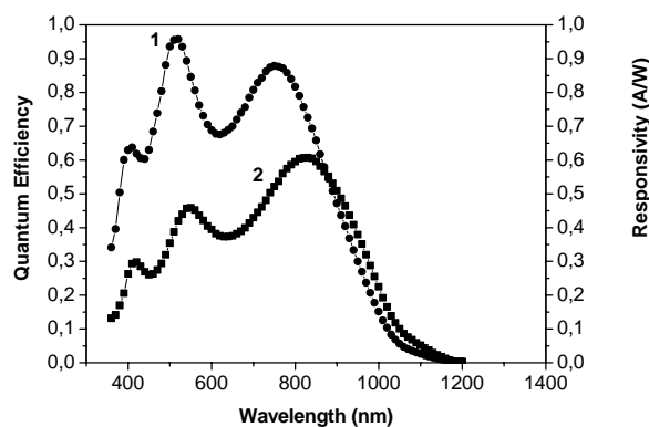
Figure 6: Spectral distribution of the quantum efficiency (1) and sensibility (2) of the n^+ITO-SiO_2-n-n^+Si solar cells.
