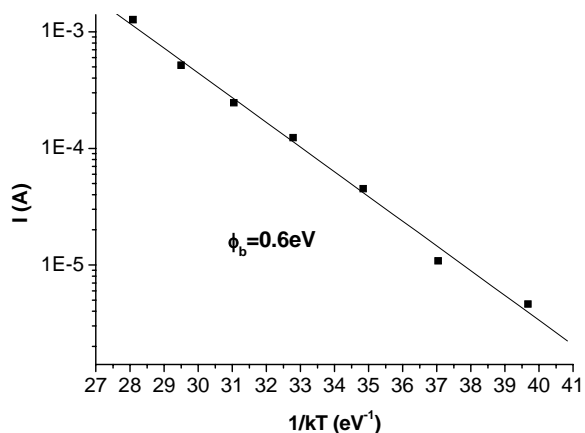
Figure 5: Dependence I_s = f(1/kT) of ITO-nSi structure.
