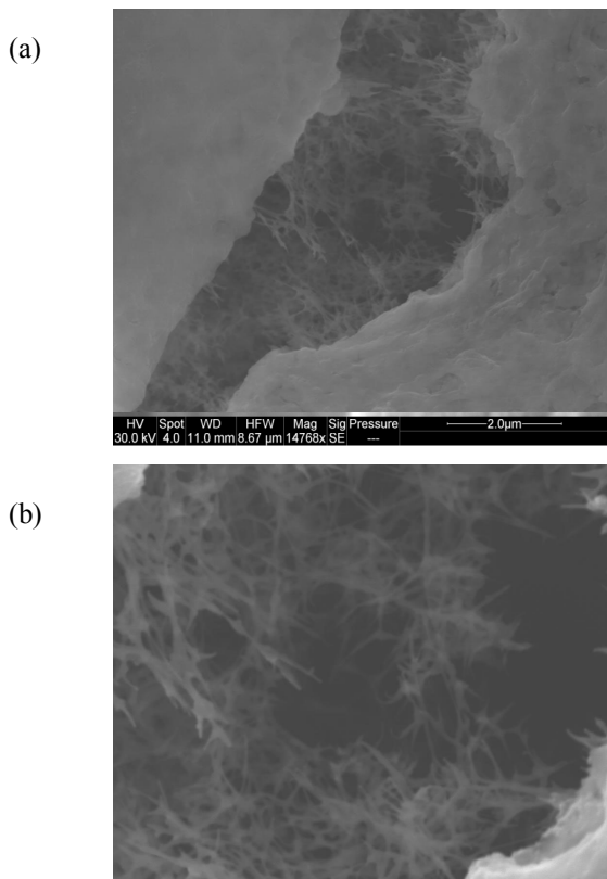
Figure 3: (a) SEM micrograph of the SWCNT thin film inside the bacterium; (b) a closer image of the SWCNT mesh thin film inside the bacterium.
