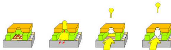
Figure 4: Inkjet process to release droplets of ink in a surface [4].
