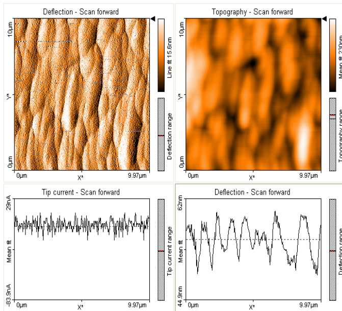
Figure 6: AFM image of the SWCNT mesh after deposited thru the inkjet nozzle on a silicon surface.
