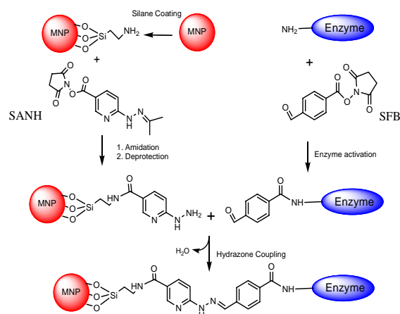
Fig. 2: Reaction scheme used for producing MNP-Es using amino-silane-coated MNP's.
