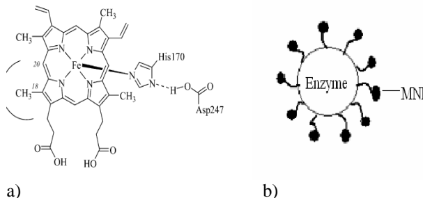
Fig. 6: a) Structure of horseradish peroxidase b) Enzyme with the envelope of MNP
