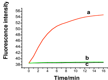
Fig.3 showed that the proton transfer was in response to the activity of F_0F_1 -ATPase by using CdTe quantum dots as indicator.
