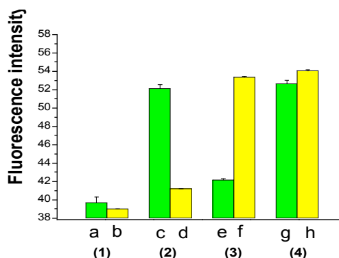
Fig. 4 the fluorescence intensity of the two types emission (535,585 nm) of CdTe quantum dots appear ability independent of each.
