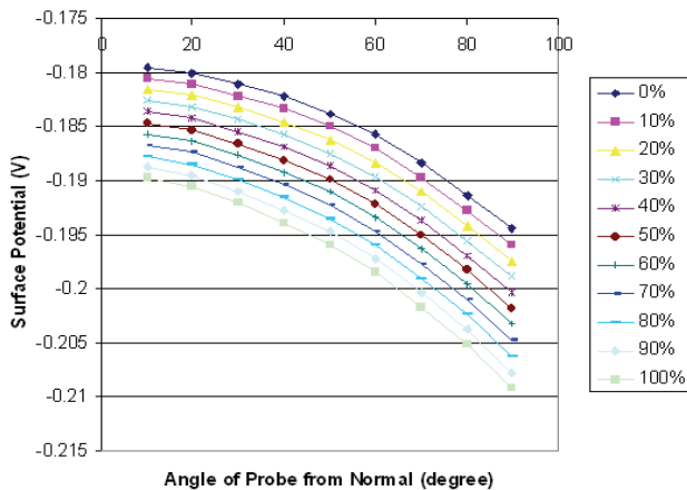
Figure 3: Surface potential as a function of angle of probe from normal and binding efficiencies.
