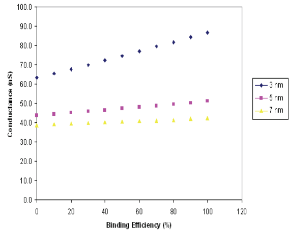
Figure 4: p-Si nanowire simulation of conductance vs. binding efficiency with 1micron gate length and 1nm oxide layer thickness at a drain voltage of 1V.
