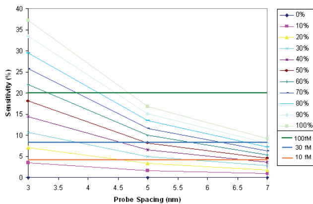
Figure 6: Sensitivity vs. probe spacing for different binding efficiencies at a constant drain voltage of 1V and oxide layer thickness of 1nm. Corresponding experimental sensitivity [1] has been added for 100 fM, 30 fM and 10 fM DNA sample for comparison.
