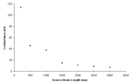
Figure 5: Conductance vs. source drain length at constant drain source voltage of 1V and 1nm oxide layer thickness.
