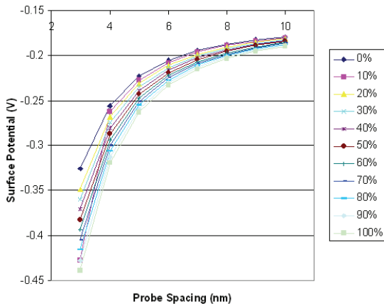
Figure 2: Surface potential on oxide layer as a function of probe spacing and binding efficiency.
