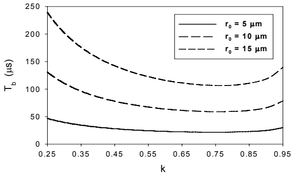
Figure 4: T_b vs. wavenumber k and jet radius.
