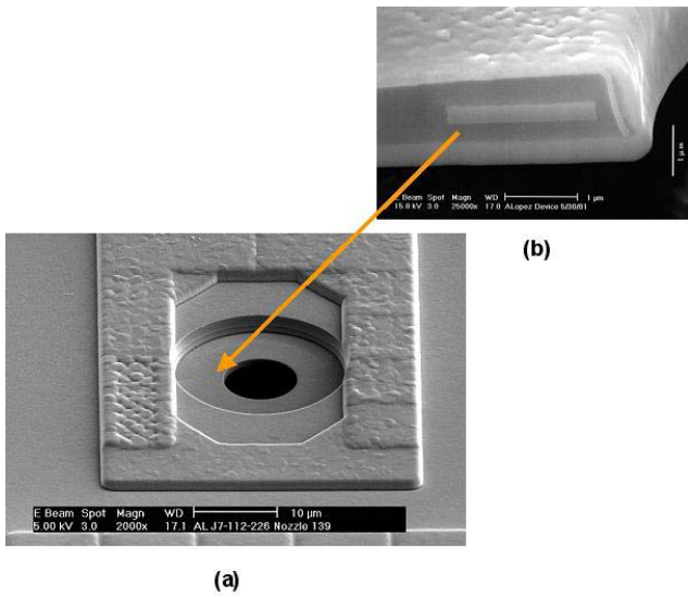
Figure 3: Nozzle with embedded integrated heater element: (a) top of nozzle, (b) cross-section of nozzle showing embedded heater.
