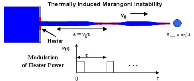
Figure 1: Illustration showing a single nozzle with an integrated heater at the orifice, and a thermal modulation pulse used to induce Marangoni instability and drop formation.
