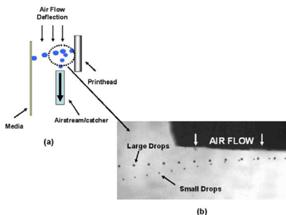
Figure 7: Continuous inkjet printing: (a) schematic showing drop size selective printing, (b) experimental picture showing airflow induced separation of large and small drops.
