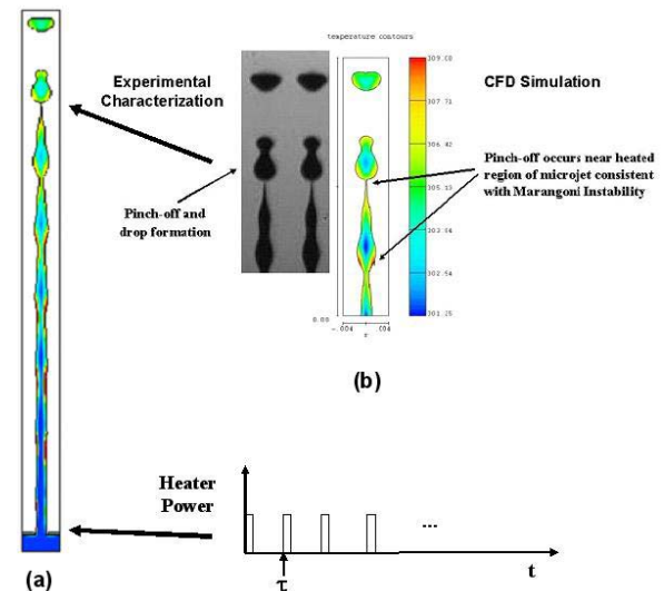
Figure 6: CFD simulation and comparison with experiment.
