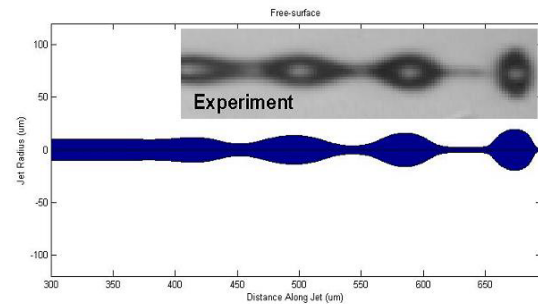
Figure 5: Slender jet analysis vs. experimental data.
