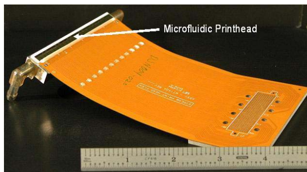
Figure 8: Fabricated microfluidic printhead.
