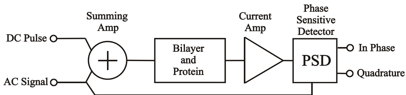
Figure 1: Block diagram of the final instrumentation set up used for phase sensitive detection of the conductances of ion channels inserted into suspended lipid bilayers. A DC holding potential and an AC reference signal are added together using a summing circuit and the resulting voltage waveform is applied to the lipid bilayer system. A low noise current amplifier is used to magnify the current response of the system to the applied potential waveform. The AC current response is compared to the reference signal of the lock-in amplifier using phase sensitive detection and the final in-phase and quadrature components are output to a text file using LabVIEW software.
