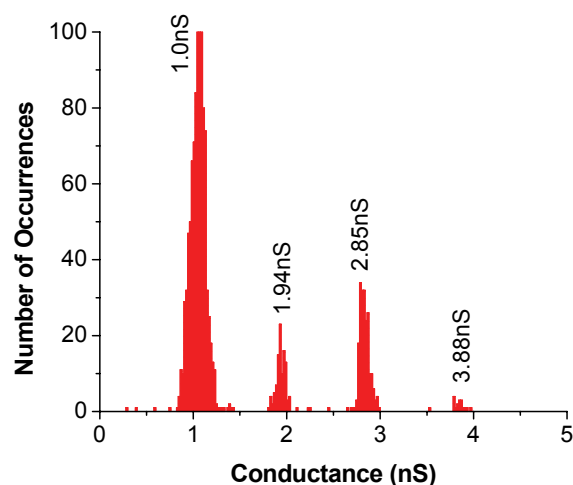
Figure 3: The bilayer and protein system conductance from Fig. 2 compiled into a histogram showing peaks corresponding to the conductance of the single channels. The average of the differences between each adjacent peak can be used to determine the average single channel conductance of the protein, in this case 0.96nS.
