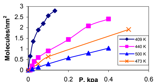
Fig. 4 Adsorption isotherm from GCMC simulation for \text{HgCl}_2 in zeolite NaX
