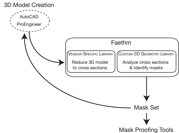
Figure 1: Implementation and integration of Faethm in a design environment.
