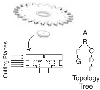
Figure 2: Locating the unique cross sections and building the topology tree for a hub which holds a gear in place.
