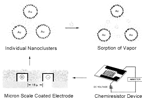
Fig. 1. MIME nanosensor concept.
