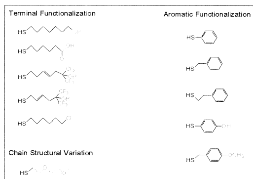
Fig. 4. Functionalized thiol ligands.
