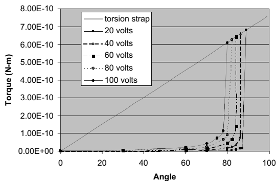
Figure 3: Electrostatics Parametric Study
