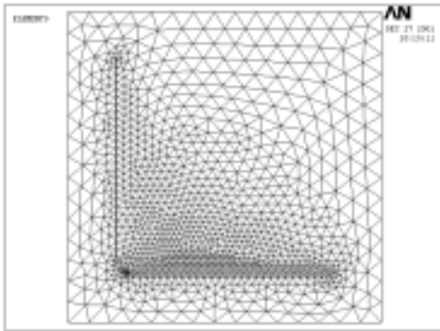
Figure 2: 2-D electrostatic elements surrounding the vertical electrode and the horizontal shutter.
