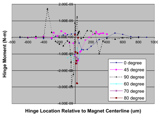
Figure 7: Hinge torque relative to the magnet's centerline.
