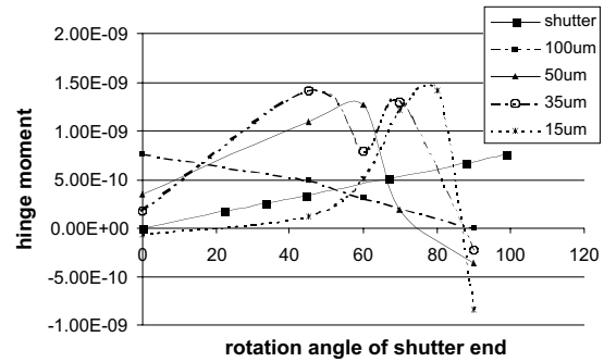
Figure 8: Shutter angle relative to distance from the magnet centerline.
