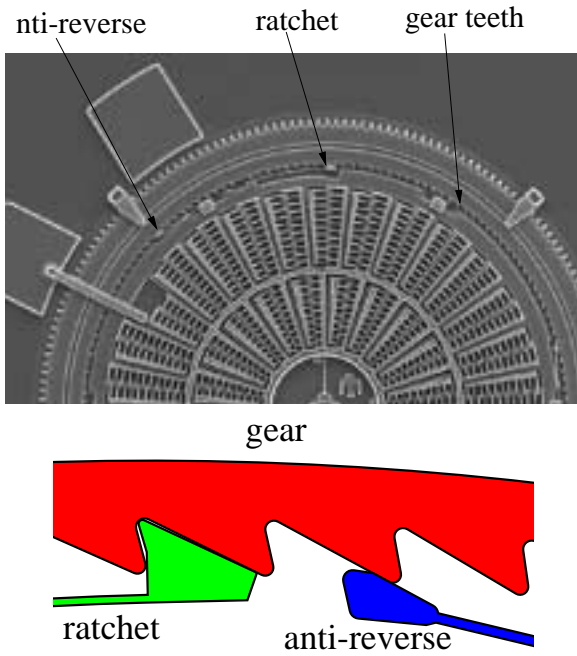
Figure 1: Torsional ratcheting actuator: (top) SEM image courtesy of Sandia National Laboratories Intelligent Micro-machine Initiative www.mems.sandia.gov ; (bottom) Detail of CAD model.
