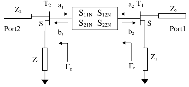
Fig. 1 Schematic diagram of a balanced oscillator incorporating a general interconnecting network
