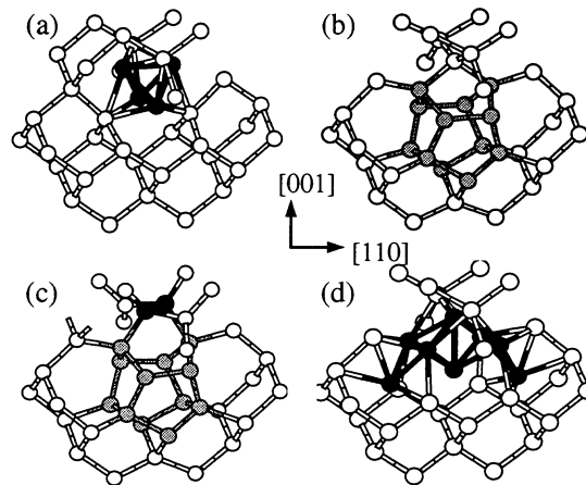
Figure 2: Core structures of compact (a) I_3 - D_{2d} , (b) I_4 - D_{2d} , (c) I_5 - C_{2v} and (d) I_5 - C_{2v} clusters extracted from collective trajectories of parallel-replica simulations using classical MEAM potential. Within ab initio LDA/GGA calculations, (a)–(c) are the lowest-energy configurations for the given size. Structure (d) is a local minimum configuration which was related to the shape transition in Ref. [12].
