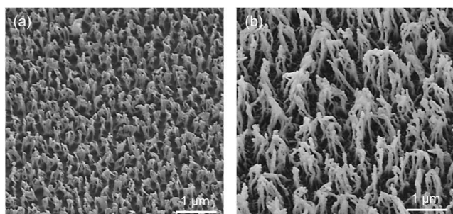
Figure 3: Tilted SEM images (30°) of O 2 plasma treated mesh for (a) 5 min, and (b) 30 min.
