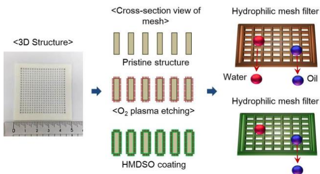
Figure 1: Schematic diagram of mesh filter preparation procedures.
