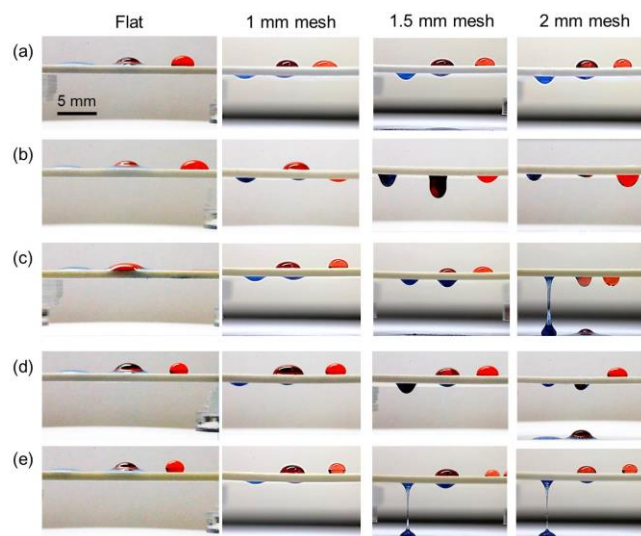
Figure 4: Oil-water separation behaviour at the different mesh filters with different pore sizes and surface functional properties. (a) Pristine, O 2 plasma etching for (b) 5 min, (c) 30 min, (d) pristine coated by HMDSO, and (e) O 2 plasma etched mesh (30 min) coated by HMDSO. Red: water, Blue: oil. The oil-water mixture was dropped at the center of each filter.
