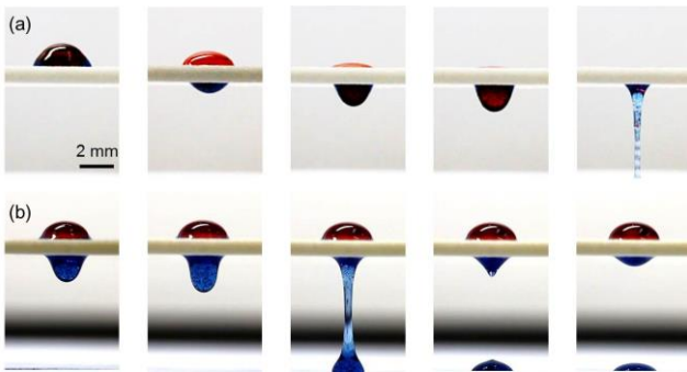
Figure 6: The dynamic motion of oil-water mixture on the (a) hydrophilic ( O_2 plasma etching for 5 min) and (b) superhydrophobic mesh filter ( O_2 plasma etching for 30 min with HMDSO coating). The pore size: 1.5 mm.
