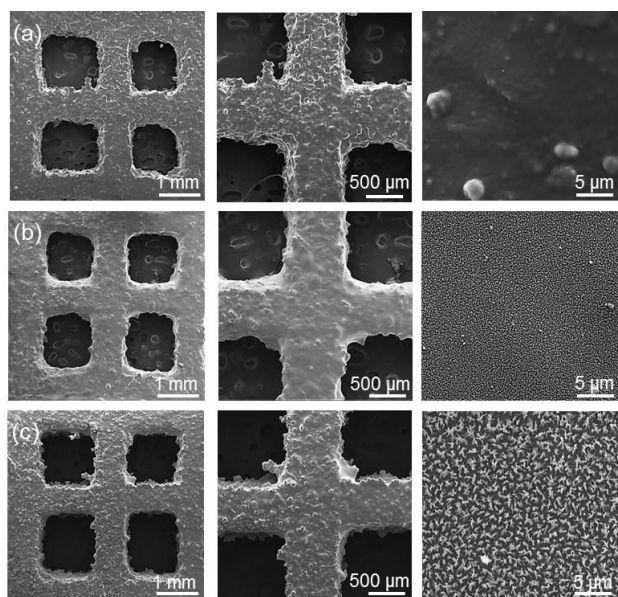
Figure 2: SEM images of (a) untreated original mesh, O 2 plasma treated mesh for (b) 5 min, and (c) 30 min. From left to right, magnification is enlarged at the center of the figure to observe the surface geometry clearly.
