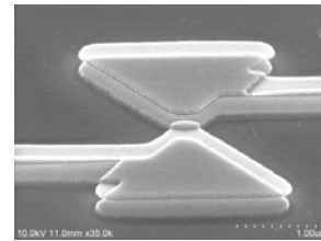
Figure 7 – Bowtie antenna and Ni-NiO-Ni MIM diode
