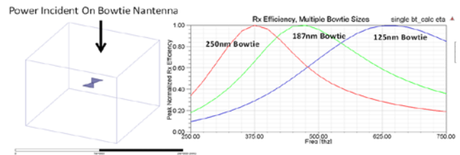
Figure 2 – Example of 3 bowtie antennas covering majority of solar spectrum
