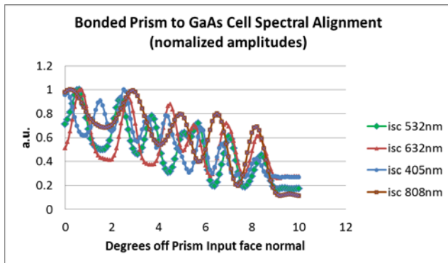
Figure 8 – Indoor angular pattern scan of 1J unit cell
