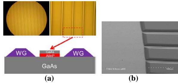
Figure 6 – a) SEM image and cross-sectional diagram of etched solar cell, b) SEM image showing 45° angle etch
