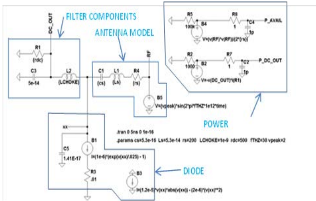
Figure 4 – LTSPICE schematic for rectenna simulation
