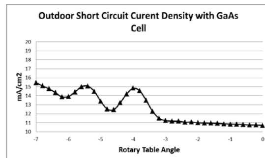
Figure 9 – Outdoor angular pattern scan of 1J unit cell
