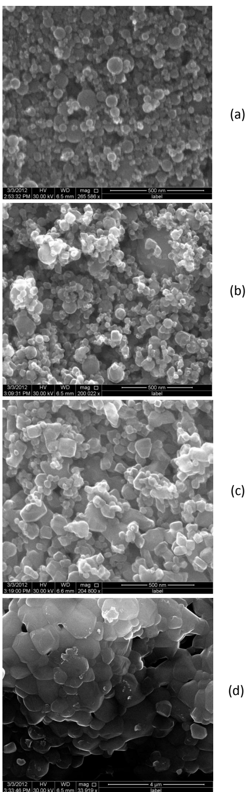
Figure 5: SEM images of nC TiO 2 powder annealed at (a) 400°C (b) 700°C (c) 800°C (d) 1000°C
