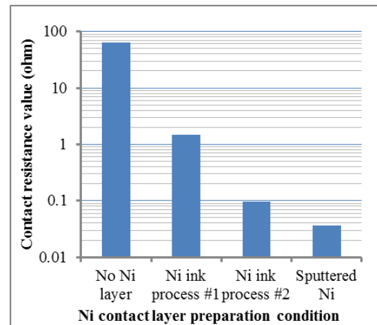
Figure 4. Measured contact resistance values for differently processed Ni contact layer.
