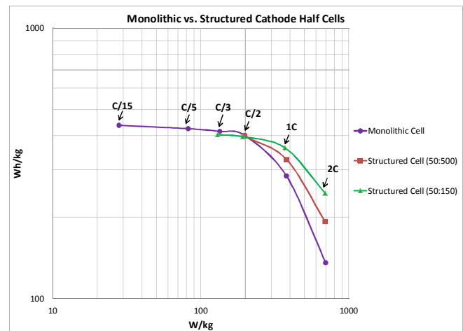
Figure 5: Modeling energy density results for interdigitated \text{LiCoO}_2 half cell batteries.
