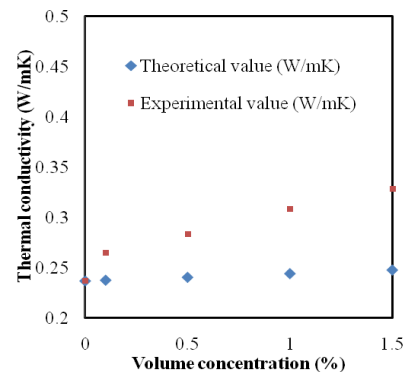
Fig.4 Variation of thermal conductivity of \text{Al}_2\text{O}_3/\text{DMAC} nanofluid with volume concentration
