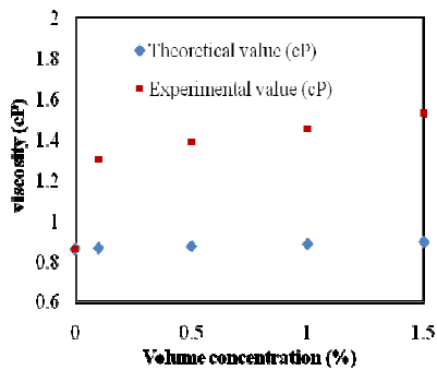
Fig.5 Variation of Dynamic viscosity of \text{Al}_2\text{O}_3/\text{DMAC} nanofluid with volume concentration
