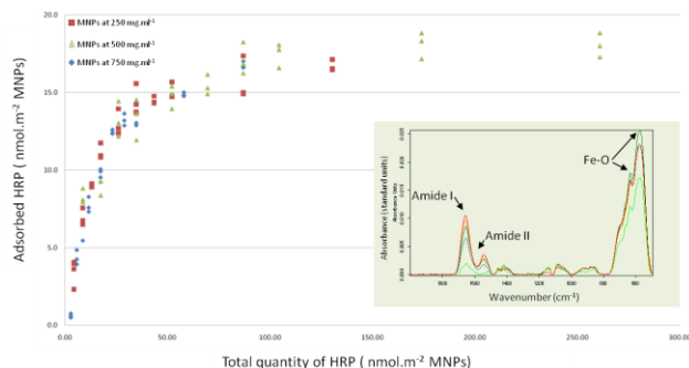
Figure 1: Quantification of entrapped Horseradish Peroxidase (HRP) by QHT-FTIR for M90 expressed as immobilized HRP standardized per total surface area. Insert: FTIR spectra of M90-BNCs used for the standardization.
