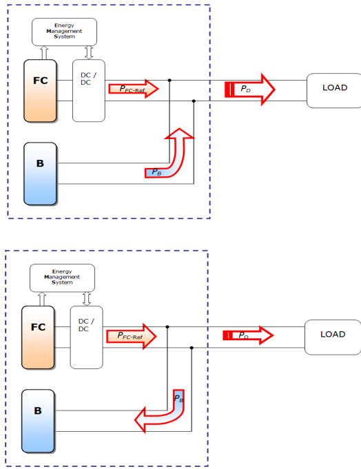
Figure 4 Operating modes of the demonstrator. Battery discharge and charge
