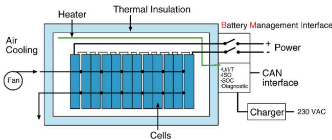
Figure 1 Fiamm SoNick battery layout
