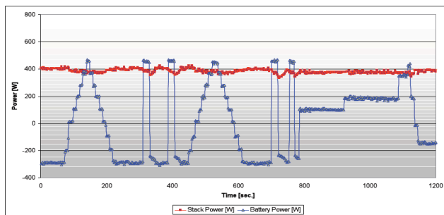
Figure 5 SOFC/ZEBRA hybrid system electrical behaviour
