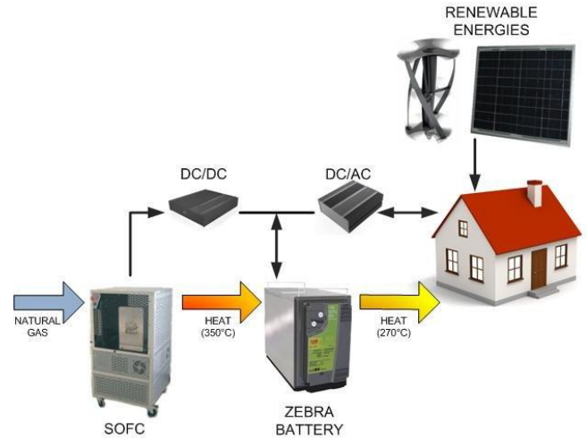
Figure 6 Scheme of integration between the \mu -CSHP developed and RWE at dwelling stage
