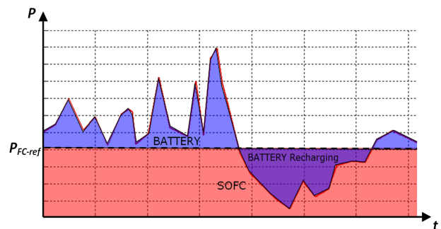
Figure 3 Example of expected power curves during operation
