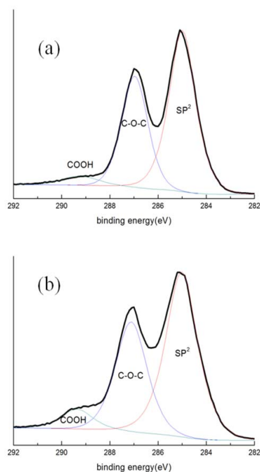
Fig 3 XPS results of GO(0) and GO(5). Each result is deconvoluted into three peaks
