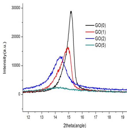
Fig 2 XRD pattern of GO samples obtained after high-energy ball milling for 1,2 and 5h
