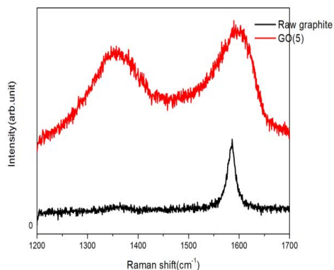
Fig 1 Raman spectroscopy result of Raw graphite and GO(5)
