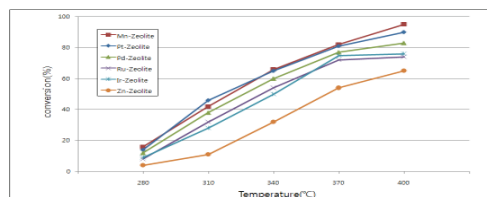
Fig. 4. PP dissociation conversion according to various catalysts.
