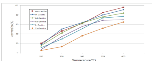
Fig. 5. ABS dissociation conversion according to various catalysts.
