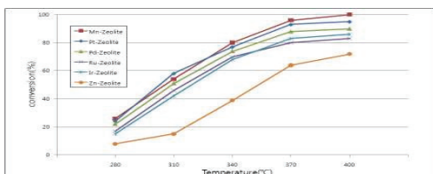
Fig. 3. PE dissociation conversion according to various catalysts.
