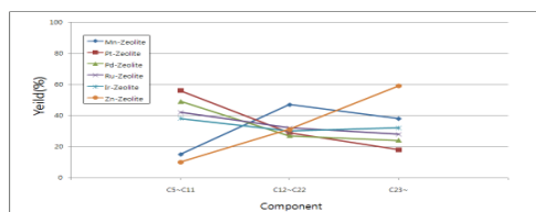
Fig. 10. Liquid product distribution of PE according to various catalysts at 400°C
