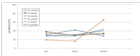
Fig. 7. Product distribution of PE at 340°C according to various catalysts.
