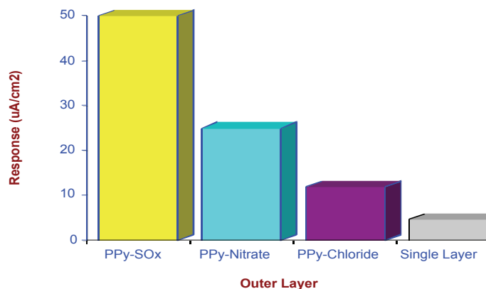
Figure 2: Influence of outer nanolayer composition on amperometric response of sulfite on a bilayer electrode. Inner layer is PPy-Dex-SOx. E app is -0.1 V.
